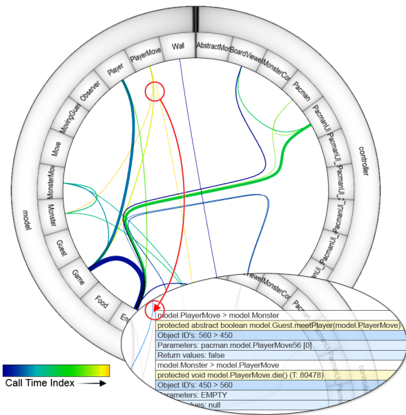
Figure 6. Circular, temporal view of the “player dies” feature that shows runtime information.
