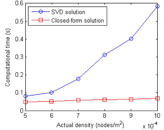
Fig. 3. Computational time of the traditional solution and the closed-form solution.
