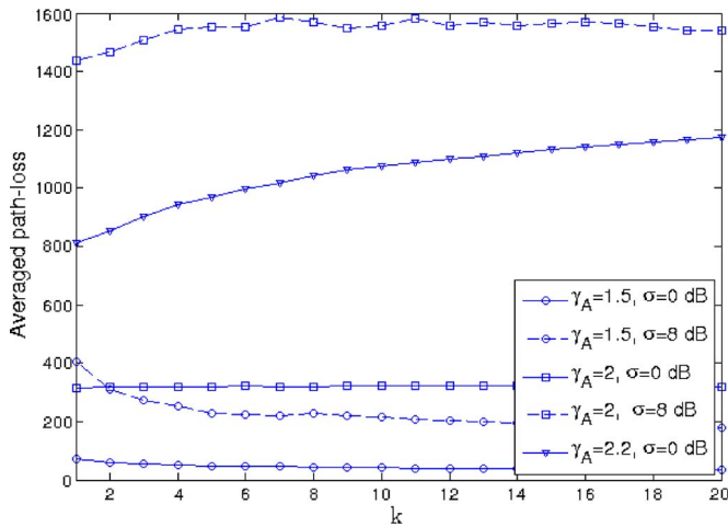
Fig. 12. Numerical results of the k th nearest neighbor routing in 2-D space.
