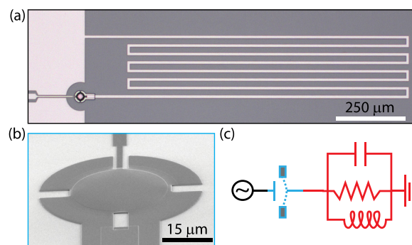
FIG. 1. Microwave cavity readout of a superconducting drum with electrostatic driving. (a) Optical microscopy image of the device. A drumhead mechanical oscillator is capacitively coupled to the microwave input port of a high impedance microwave cavity on a sapphire substrate. (b) Scanning electron microscopy image of the MoRe drumhead resonator. The drum is 30 \mu\text{m} in diameter and is suspended approximately 290 nm above the gate bottom electrode. (c) Device schematic diagram: the mechanical drum is capacitively coupled to the microwave input port. Motion of the drum modulates both the resonance frequency \omega_c and the external coupling rate \kappa_e of the cavity.
