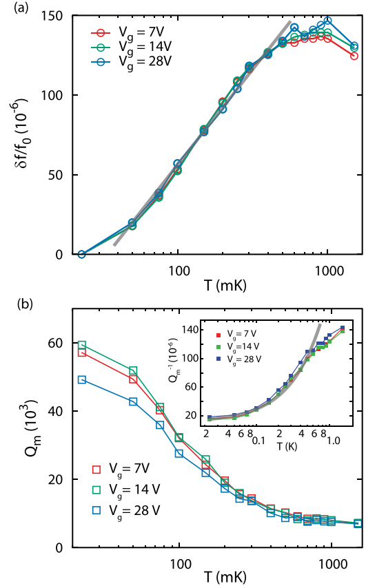
FIG. 3. Temperature dependence of (a) normalized relative frequency shift \delta f = (f_0(T) - f_0(23 \text{ mK}))/f_0(23 \text{ mK}) and (b) the mechanical quality factor. The mechanical quality-factor is determined from fitting to a Lorentzian function. Measurements are taken at three different voltages 7, 14, and 28 V. The inset shows the plot of inverse quality-factor Q_m^{-1} . The gray lines are the numerical fits to the data.
