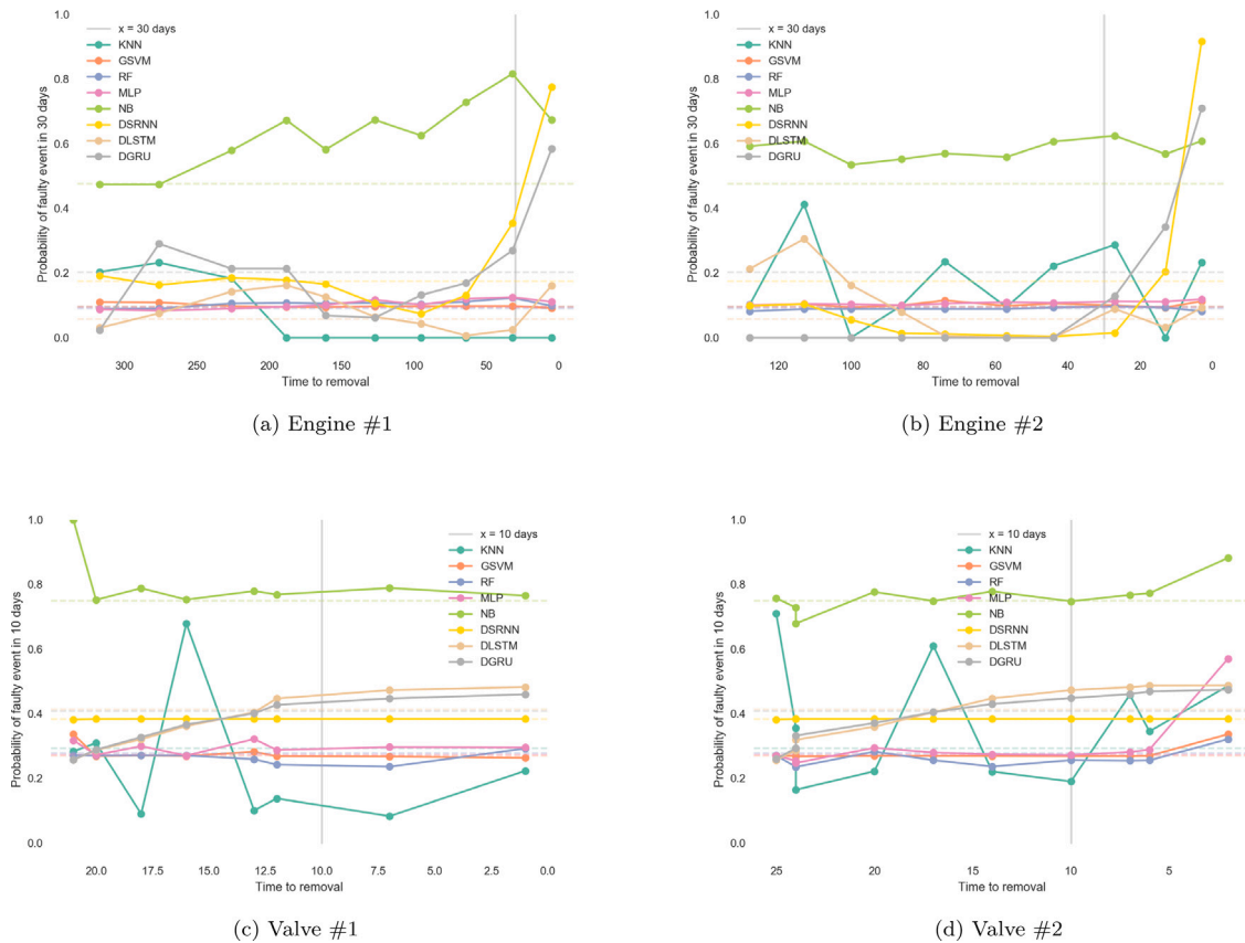
Fig. 8. Performance of classifiers on randomly selected overhauls on dataset DS-1 and randomly selected valves on dataset DS-2.
