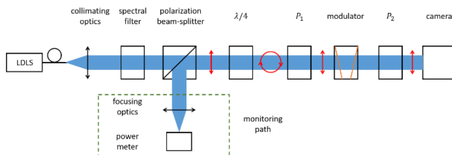
Figure 5-1. Scheme of the polarisation characterisation measurement setup, the beam is pictured in blue, the red arrows represent the polarisation at different places of the beam.
