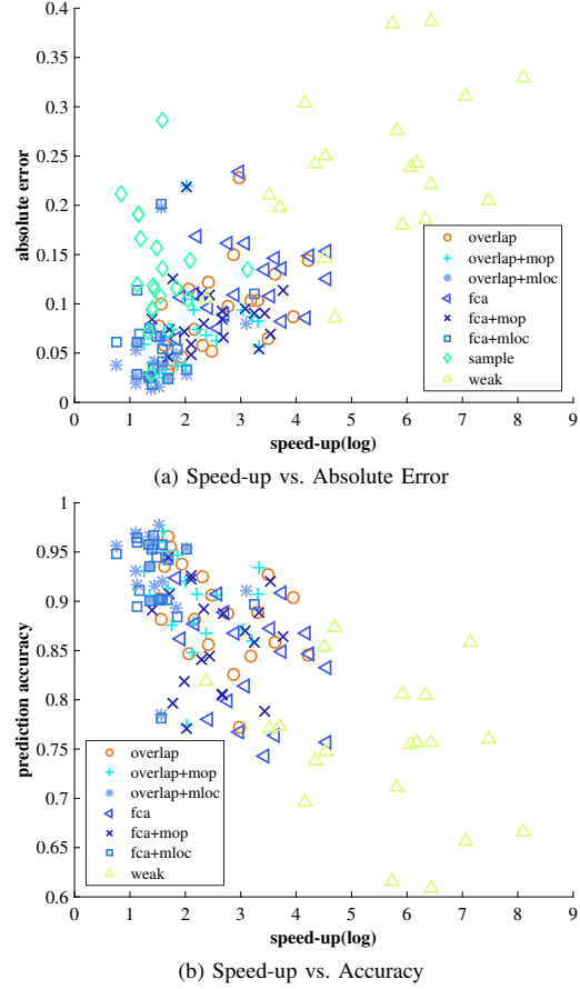
Fig. 3. Graphical comparison of the eight mutation strategies in terms of speed-up, absolute error and accuracy.
