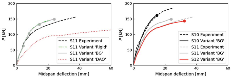
Fig. 4. Load-deflection curves of the experiments and NLFEAs. Left: test S11 and the predictions from three interface shear models. Right: tests S10–S12 and the predictions from the “best-guess” interface shear model. The experimental load-deflection curve of S12 was not reported in [9].
