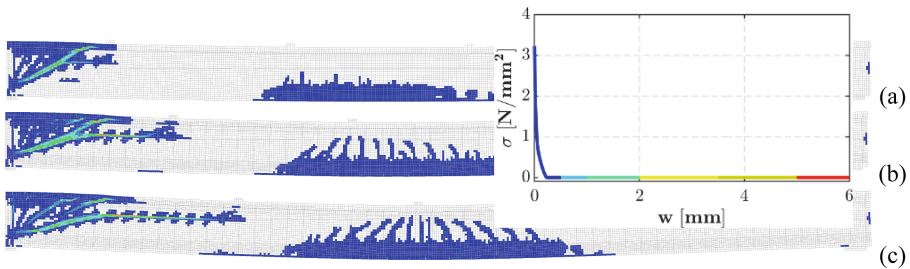
Fig. 6. Crack width plot in a deformed mode (with amplification factor: x5) at the last converged steps of the “best-guess” analyses of test S10 (a), S11 (b) and S12 (c).
