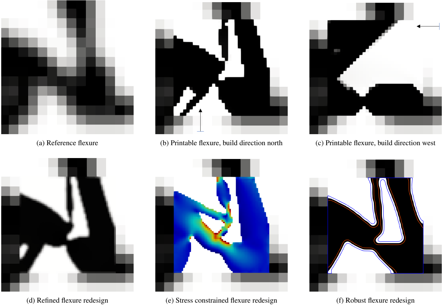
FIGURE 5: A variety of refined redesigned flexures with varying refinement ratios and DfAM constraints.
