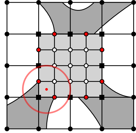
FIGURE 3: Reinitialization of redesign domain. The structural DOFs are separated in three sets, the DOFs in the redesign domain ( \circ ), non-design domain ( \bullet ) and interface ( \blacksquare ) regions. Some redesign DOFs ( \bullet ) are coupled to the interface DOFs using MPCs. Note that for some design variables the filter radius (both for density and overhang filter) exceeds outside of the redesign domain, as indicated by the red circle.
