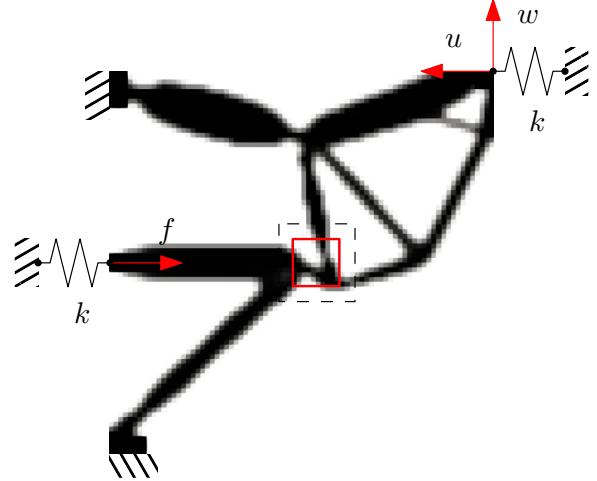
(b) Topology resulting from solving Eq. (11).
