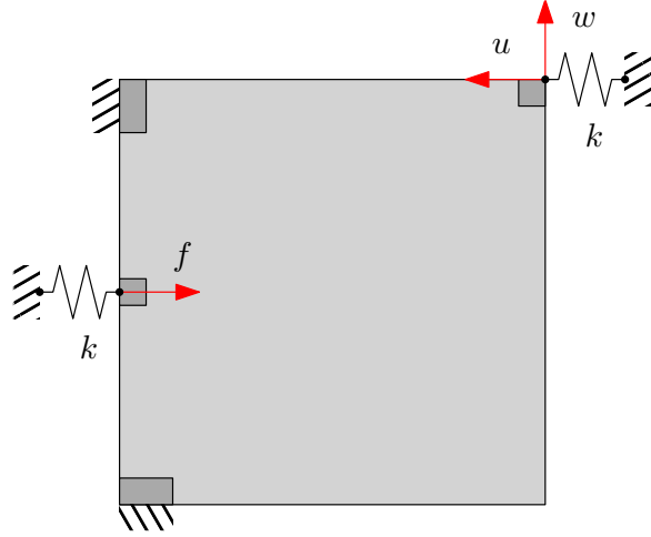
(a) Design domain and boundary conditions. The domain is discretized in 80 by 80 square quadrilateral finite elements.
