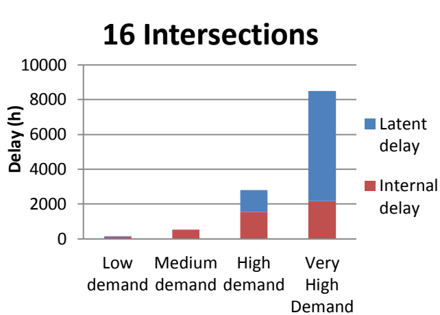
Figure 5-14: Internal and latent delay sixteen intersections
