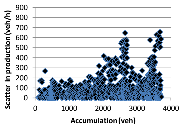
Figure A-4: Absolute scatter deviation of MFD with an applied maximum deviation factor of 0,1 and different desired perimeter flows for intersections with two and three adjacent intersections
