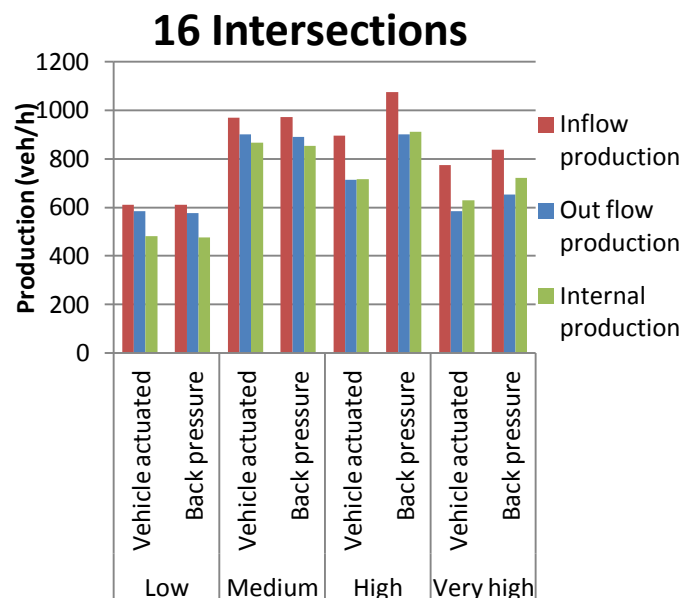
Figure 5-33: Inflow, outflow and internal production sixteen intersections
