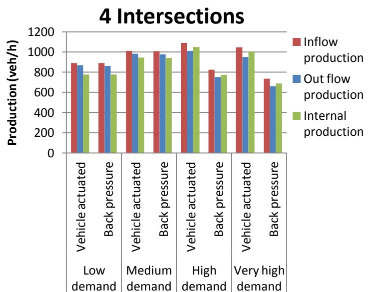
Figure 5-29: Inflow, outflow and internal production four intersections
