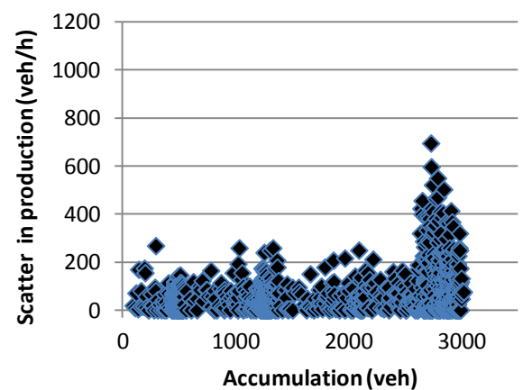
Figure 5-24: Absolute scatter deviation of all data points MFD subnetwork layout consisting of sixteen intersections
