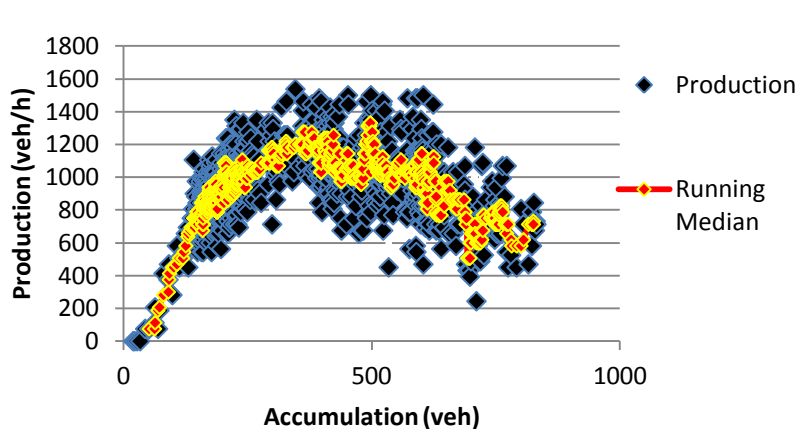
Figure 5-2: Running median of MFD subnetwork layout consisting of four intersections
