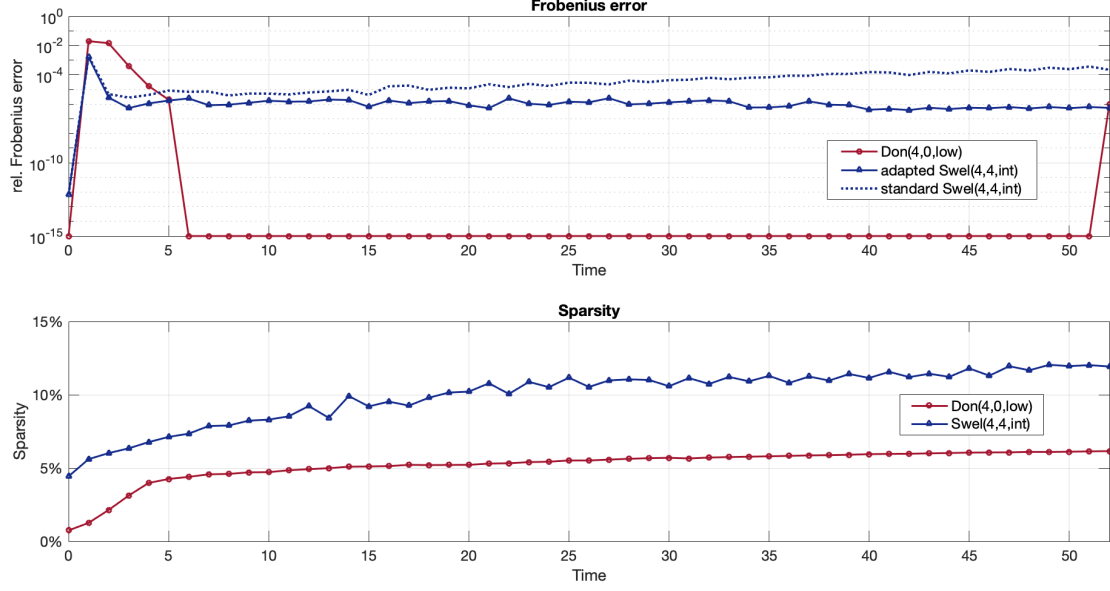
Figure 5: Version 3, error and sparsity for 2D SLV 17.
