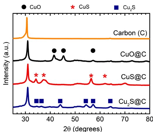
Fig. 1. X-ray diffractograms of the bare GNP-500 carbon support (orange) and of the \text{CuO@C} (black), \text{CuS@C} (red) and \text{Cu}_2\text{S@C} (blue) nanoparticles on this carbon support. All samples have a loading of 20 wt% Cu. The symbols above the diffractograms represent reflections of CuO (black dot), CuS (red asterisk) and \text{Cu}_2\text{S} (blue square), obtained from the PDF reference cards PDF-01-070-6831 (ICDD, 2019), PDF-00-006-0464 (ICDD, 2019) and PDF-00-053-0522 (ICDD, 2019), respectively. For interpretation of the references to colour in this figure legend, the reader is referred to the web version of this article.[29]
