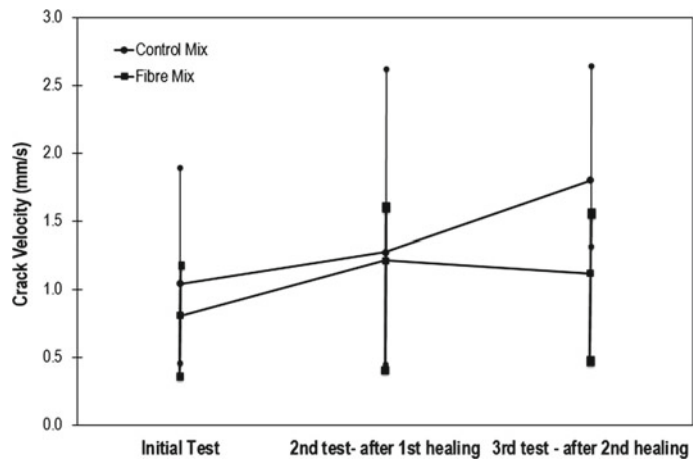
Fig. 6 Crack speed
