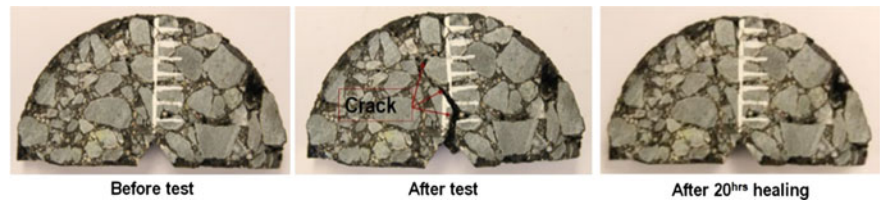
Fig. 5 SCB test specimen crack closure/healing
