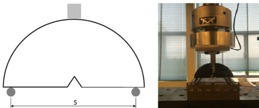
Fig. 3 Left: schematic of a SCB test specimen; right: the SCB test system set up
