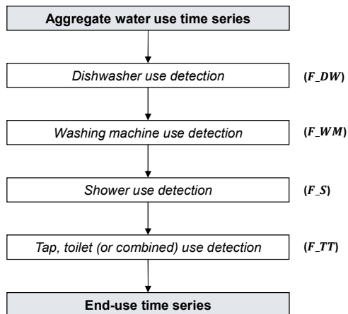
Fig. 1. Structure of the automated methodology for water end-use disaggregation.
