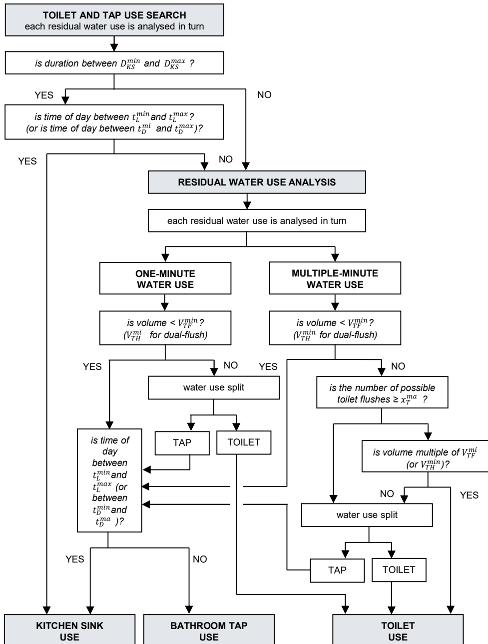
Fig. S3. Function for toilet and tap use detection ( F_{TT} ) flow chart.
