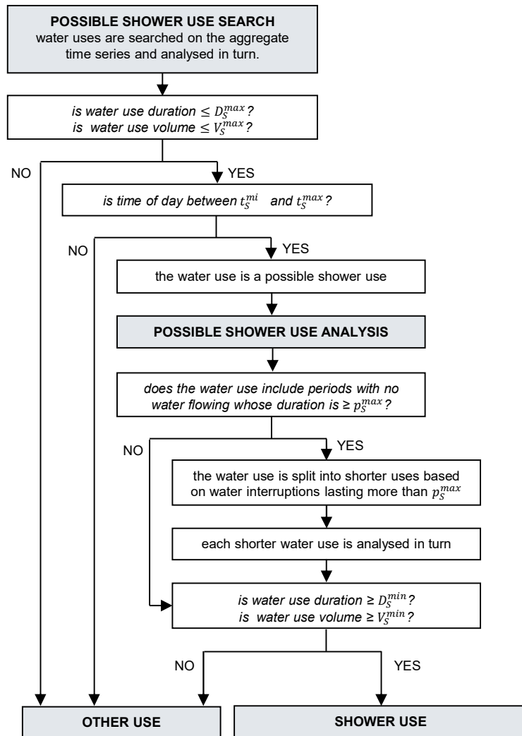
Fig. S2. Function for shower use detection ( F_S ) flow chart.
