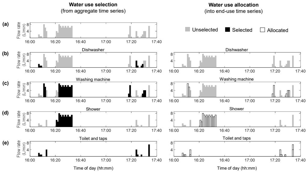
Fig. 2. Example of application of the automated methodology. Each panel (a – e) in the figure corresponds with steps a – e described in the Methods section ( Disaggregation Methodology sub-section)
