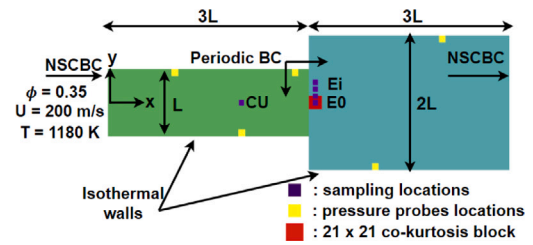
Fig. 1. Geometry of the reheat combustor shown in the mid- z plane. L = 1 cm [20].
