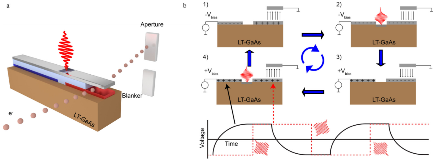
Fig. 2. (a) Schematic indication of our UFB concept: a photoconductive switch is connected to an electrostatic beam blanker, the electron beam is deflected and intercepted by an aperture, the colors of the electrodes indicate +10V (blue), negative –10V (red) and ground (grey). (b) Full modulation cycle for the UFB: (1) the beam is initially blanked by the deflection field in the blanker; (2) laser irradiation provides a conductive channel in the GaAs wafer inverting the voltage on the deflector and thus the deflection direction; (3) after the laser pulse, the GaAs restores to its insulating state, subsequently the bias on the feed voltage from the supply line is switched; (4) a next laser pulse again inverts the field in the deflector, sweeping the beam in opposite direction, after which the voltage supply inverts again and the modulation cycle is back to the initial situation. (For interpretation of the references to colour in this figure legend, the reader is referred to the web version of this article.)
