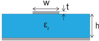
Fig. 11. Microstrip line with electrode separation h , in our case 1 \mu\text{m} , the width, w , is equal to 30 \mu\text{m} . The dielectric has a relative permittivity \epsilon_r .
