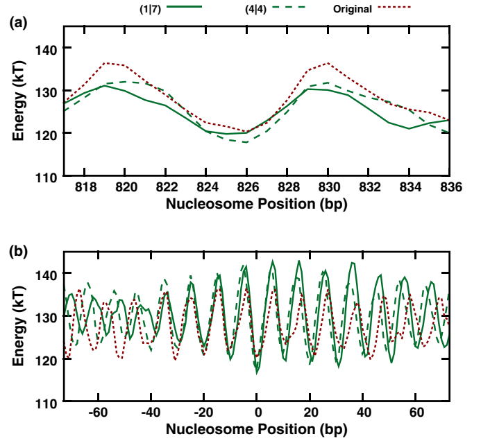
FIG. 4. (a) Nucleosome energy landscapes in a small neighborhood of position 826 of the YAL002W gene, with the 826-sequence replaced by the sequences found through SynMMC at states (1|7) and (4|4). In each case, the replacement sequence still provides a local minimum. (b) Cyclical energy landscapes of sequences found through free MMC for states (1|7) and (4|4) compared to the sequence at position 826 of the YAL002W gene. There remains always a strong local minimum at position 0.
