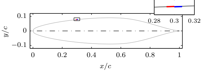
Figure 1: Schematic (to scale) of the airfoil (orthogonal to the wing leading edge) used in the present work with the AC-DBD actuator installed at x/c = 0.30 . Inset: detailed view of the actuator. Red line: exposed electrode; blue line: covered electrode.
