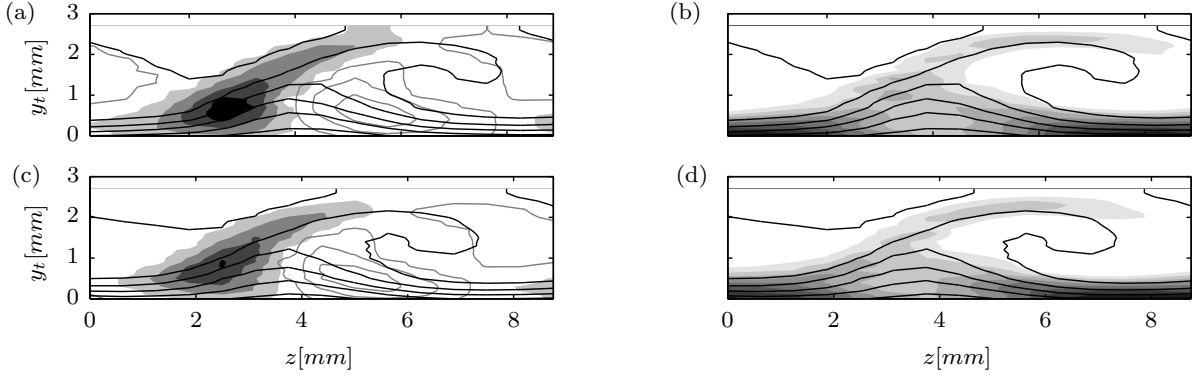
Figure 16: (a and c) non-dimensional spanwise velocity gradient ( (\partial|\bar{V}^{HWA}|/\partial z)/(|\bar{V}_e^{HWA}|/\lambda_z) ) (10 levels, shaded: between -37.4 and -3.74 ; grey solid lines: between 3.74 and 37.4 ); (b and d) non-dimensional wall-normal velocity gradient ( \partial|\bar{V}^{HWA}|/\partial y_t/(|\bar{V}_e^{HWA}|/\lambda_z) ) (10 levels, shaded from 20.79 to 207.9 ). (a and b) stronger CFV; (c and d) reduced amplitude CFV. Black line contours denote time averaged velocity.
