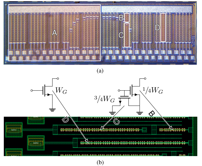
Fig. 6. Layouts of the segmented LDMOS power die. (a) Micrograph of the die (4.9 mm \times 1.6 mm) having a total gate width ( W_{G,\text{tot}} ) of 41.472 mm distributed over two switch banks (the surrounding box indicates the left switch bank A), each bank featuring seven binary-weighted segments, (B) indicates such a binary segment with dummy device (C), and 15 unary segments representing 4 bit, denoted by D. (b) Layout detail showing the use of a dummy LDMOS device (C) for equalizing C_{in} = C_{ESD2} + C_{GS} + C_{GG,dummy} . Here, the second MSB binary segment is shown below a unary segment.
