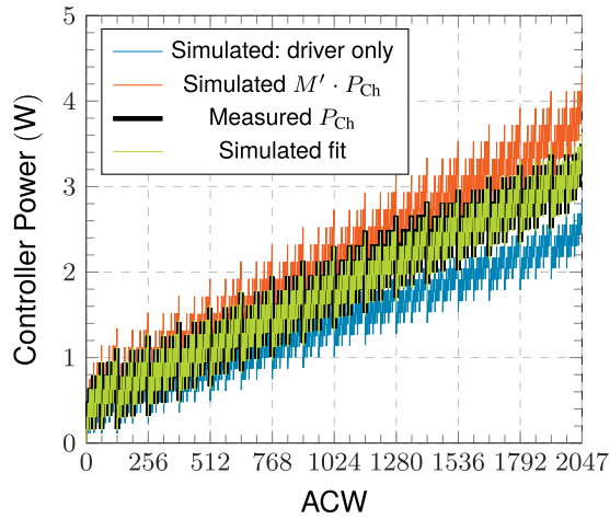
Fig. 10. Simulated drive power including C_{dr,01} , this power is multiplied by the theoretically calculated M' = 1.532 to provide the total power consumption of the driving drive chain, which is compared to its actual measured values.
