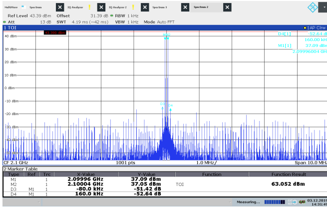
Fig. 15. Measured spectrum of the 80-kHz two-tone signal, showing an \text{IM}_3 \leq -51.4 dBc after static DPD, only using the unary segments with pulse density modulation.
