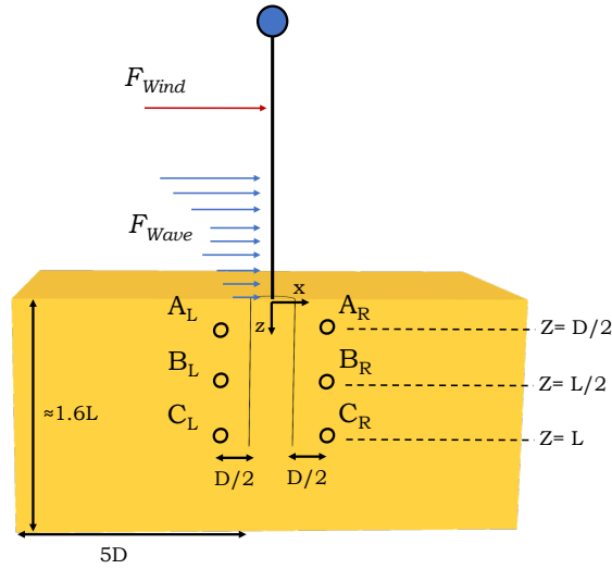
Figure 4: OWT model and location of the control points A_{L,R} , B_{L,R} , C_{L,R} within the soil domain.
