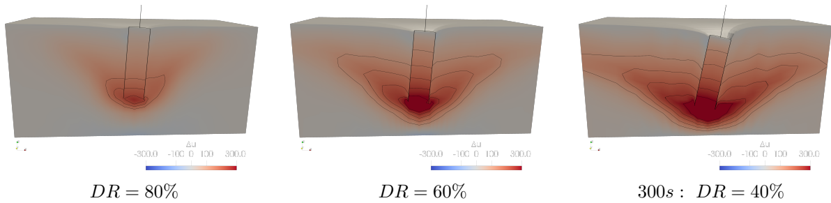
Figure 6: Excess pore pressure contour plots at 300 s of Case B for D_r = 80\% , 60\% and 40\% . Colorbars indicate \Delta u in the range [-300 kPa; 300 kPa].
