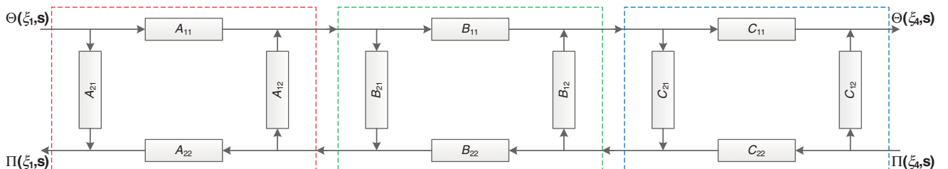
Fig. 7—Coupled model in block-diagram representation for the model depicted in Fig. 6.
