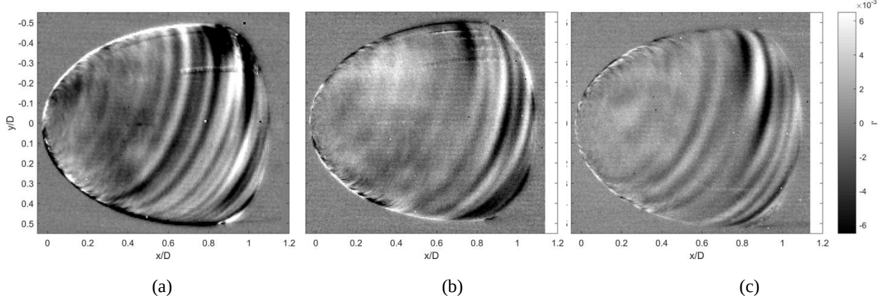
Figure 12 Instantaneous reconstruction (using 5 th to 50 th POD modes) of the spiral vortices on the rotating ellipsoid (a) \alpha = 0^\circ , (b) \alpha = 10^\circ counter rotating side, and (c) \alpha = -10^\circ co-rotating side. ( S_b = 5, Re_D = 7.7 \times 10^3 ).
