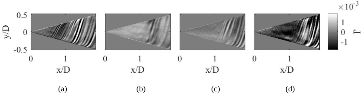
Figure 5 Delayed formation of the coherent spiral vortices under an incidence angle (a) \alpha = 0^\circ , (a) \alpha = 2^\circ , (a) \alpha = 4^\circ and (a) \alpha = 10^\circ , ( S_b = 5, Re_D = 7.7 \times 10^3 ).
