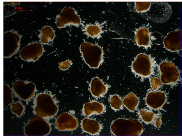
Figure 4. Granules after 120 days in the reactor in period 4.
