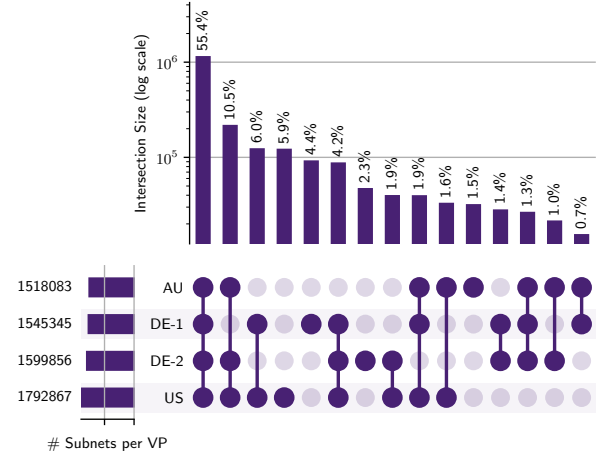
Figure 2: Upset plot of subnets discovered per vantage point using the ICMP Echo-based method.
