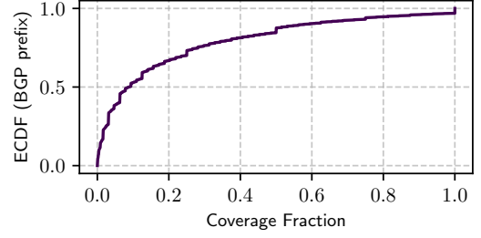
Figure 4: ECDF of subnets coverage in BGP prefixes.
