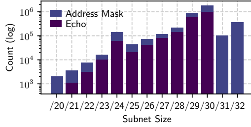
Figure 3: Number of detected subnets per size and method.
