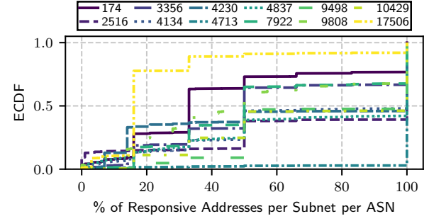
Figure 6: % of ICMP Echo replies for top ASNs.
