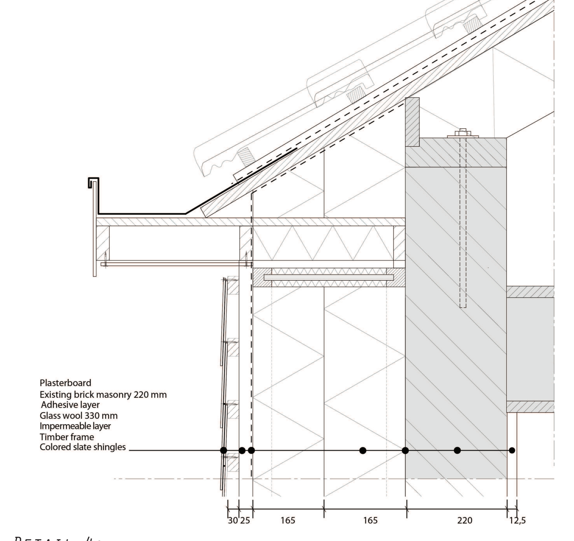
DETAIL 4: ROOF DETAIL OUTSIDE INSULATION 1:5
