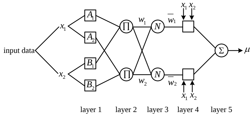
Figure 1. ANFIS structure.
