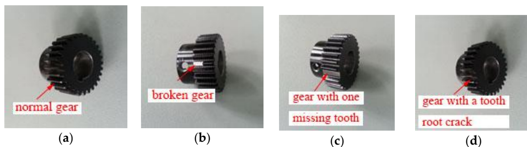
Figure 3. Four types of gears, (a) normal gear, (b) broken gear, (c) gear with one missing tooth, (d) gear with a tooth root crack.
