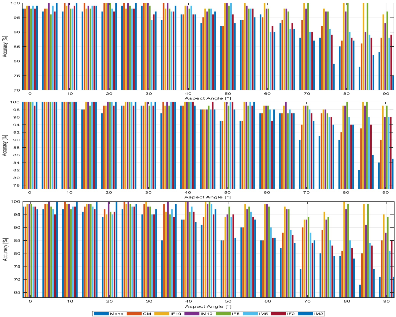
FIGURE 7 Comparison of the accuracy of the eight geometries (mono, CM, IF10, IM10, IF5, IM5, IF2, IM2) for: (a) activity IV—the IF configuration dominates or equates IM in high aspect angles (>50°) and at 45°, and IM dominates or equates IF up to 40° and at 50°, (b) activity V—the IF configuration dominates or equates IM in high aspect angles (>40°) except at 55° and 65° where IM dominates, and IM dominates or equates IF up to 40° and (c) activity VI—the IF configuration dominates or equates IM in high aspect angles (>40°), and IM dominates or equates IF up to 40° for the scenarios where the aspect angle changes from 0° to 90° with 5° steps
