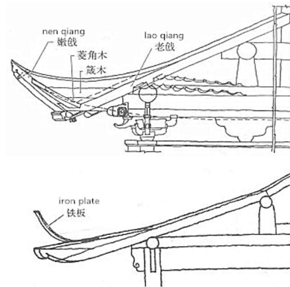
FIG. 4.15 Structural diagrams of Nén Qiāng Fa Qiāng and Shuǐ Qiāng Fa Qiāng (Illustration of Chinese classical architecture 中国古典建筑图释)
