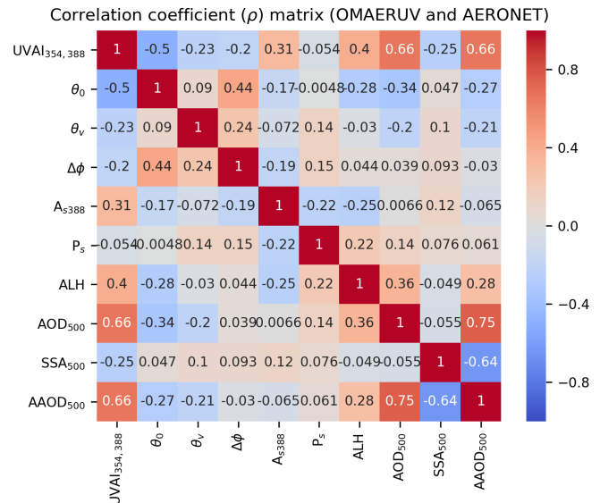
Figure 6. Spearman rank correlation coefficient matrix ( \rho ) of parameters in the OMAERUV–AERONET joint data set.
