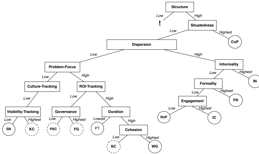
Fig. 2 A decision-tree for organisational structures - dotted nodes identify types not currently implemented in YOSHI .
