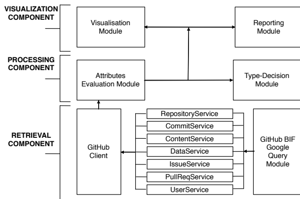
Fig. 5 YOSHI high-level architecture.
