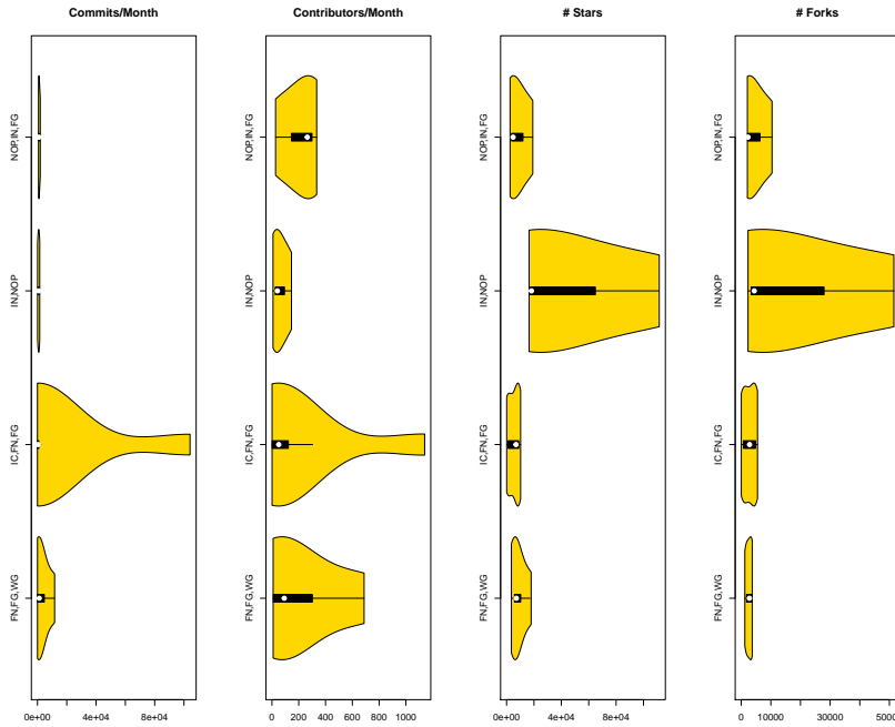
Fig. 8 Violin Plots reporting the repository health metrics for each community type inferred by YOSHI
