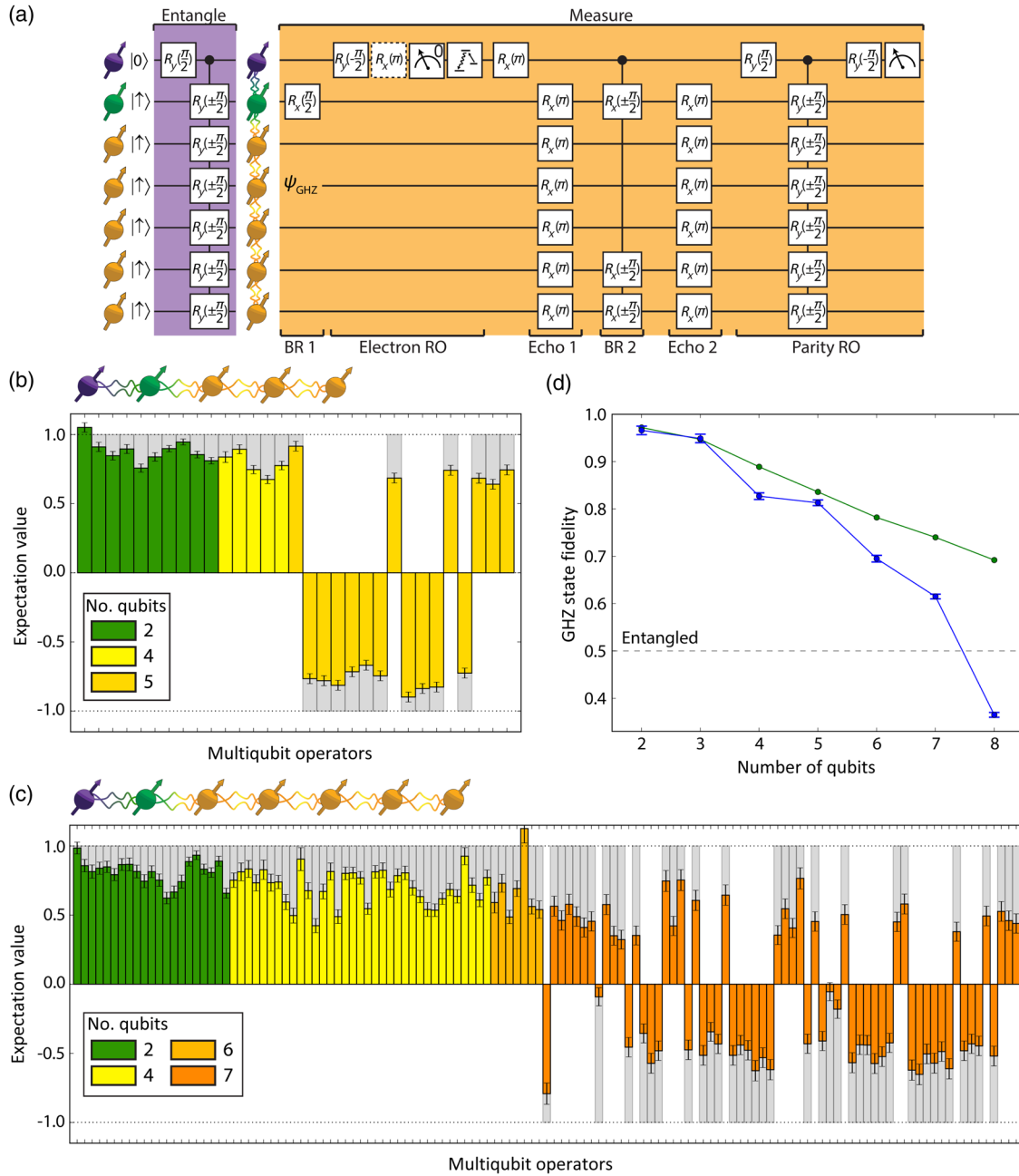
FIG. 7. (a) Experimental sequence to prepare a seven-qubit GHZ state |\text{GHZ}_7\rangle (purple) and determine the expectation value of the seven-qubit operator XYZZZZ (orange). The measurement sequence is broken down into basis rotations (BR 1,2), an electron readout (RO), nuclear spin echoes (echo 1,2), and a multiqubit readout of the nuclear spins. All operations are applied sequentially (in the same way as shown in Fig. 5), but some are shown in parallel for clarity. (b),(c) Bar plots showing the measured expectation values (nonzero terms of the ideal state only) after preparing the five-spin (b) and seven-spin (c) GHZ states. The colors indicate the number of qubits involved, i.e., the number of (nonidentity) operators in the expectation value (inset). Gray bars show the ideal expectation values. See the Supplemental Material [53] for the operator corresponding to each bar. The fidelity with the target state is 0.804(6) (b) and 0.589(5) (c), confirming genuine multipartite entanglement in both cases. (d) Plot of GHZ state fidelity against the number of constituent qubits. A value above 0.5 confirms genuine N -qubit entanglement. The blue points are the measured data, while the green points are theoretical predictions assuming a simple depolarizing noise model whose parameters are extracted from single- and two-qubit experiments. Numerical values are given in the Supplemental Material [53].
