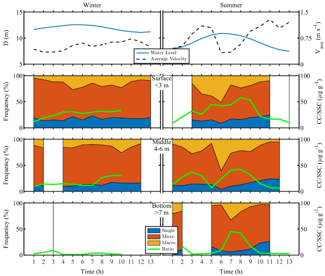
Figure 10 Time series of three floc fractions with CC/SSC ratio in winter and summer season in surface, middle and bottom water layers
