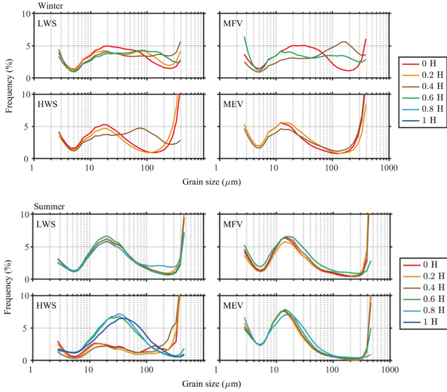
Figure 6 Vertical variations of floc size distribution measured by LISST in different tidal phases, at neap tide.
