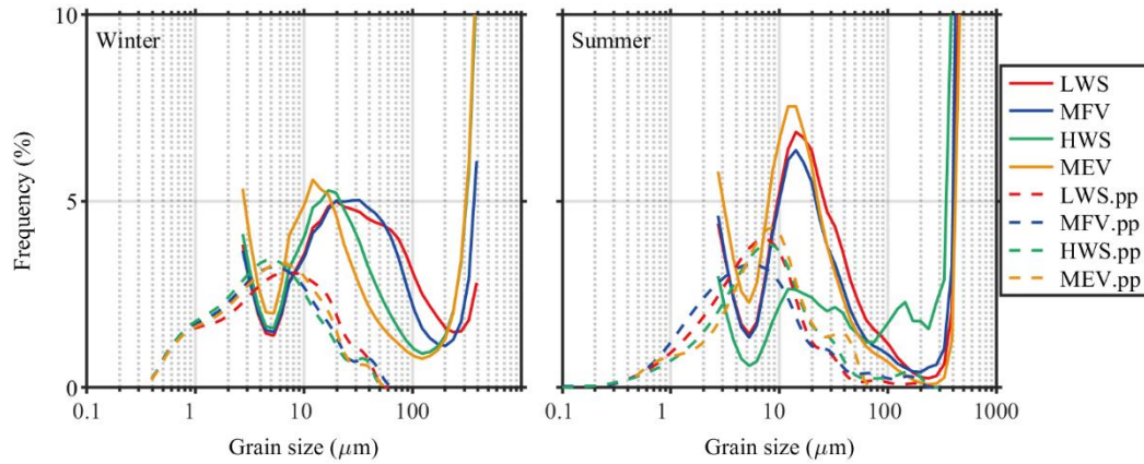
Figure 8 Surface water size distribution of both dispersed (“pp”, i.e. measured in the lab after deflocculation) and flocculated particles (as measured in-situ) in different tidal phases.
