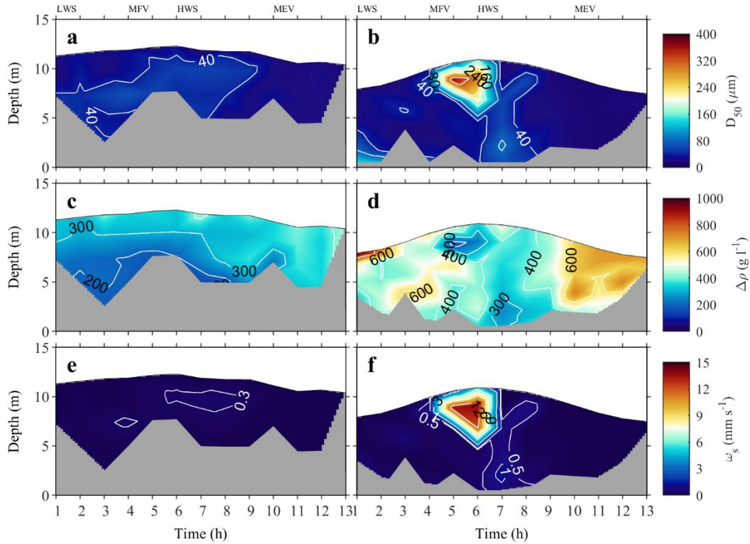
Figure 3 Vertical distribution of mean floc size (a, b), effective density (c, d) and settling (e, f) velocity. (Left: 2014-01 winter season, Right: 2016-07 summer, LWS: 1–2 h, MFV: 4–5 h, HWS: 6–7 h, MEV: 10–11 h)
