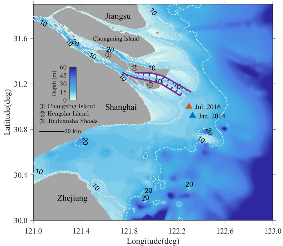
Figure 1 Map of the morphology of the Changjiang estuary and the study sites in summer (July in 2016) and winter (January in 2014).
