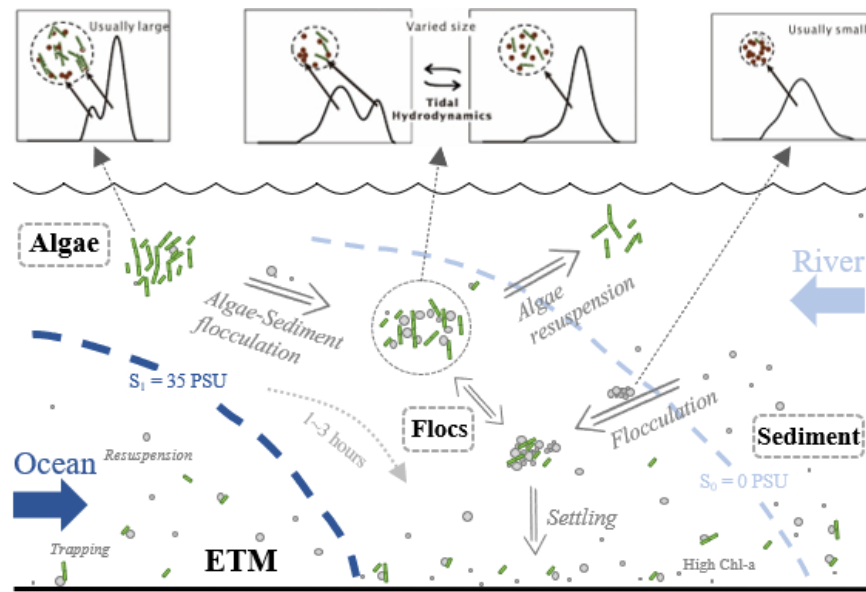
Figure 12 Algae-Sediment flocculation processes in estuary
