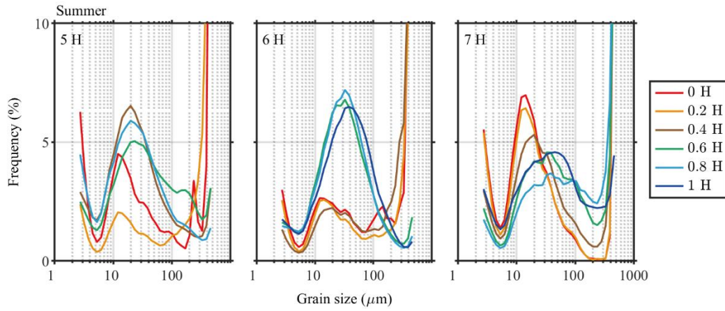
Figure 7 Vertical variations of flocs PSDs in summer during the period 5–7 hours.
