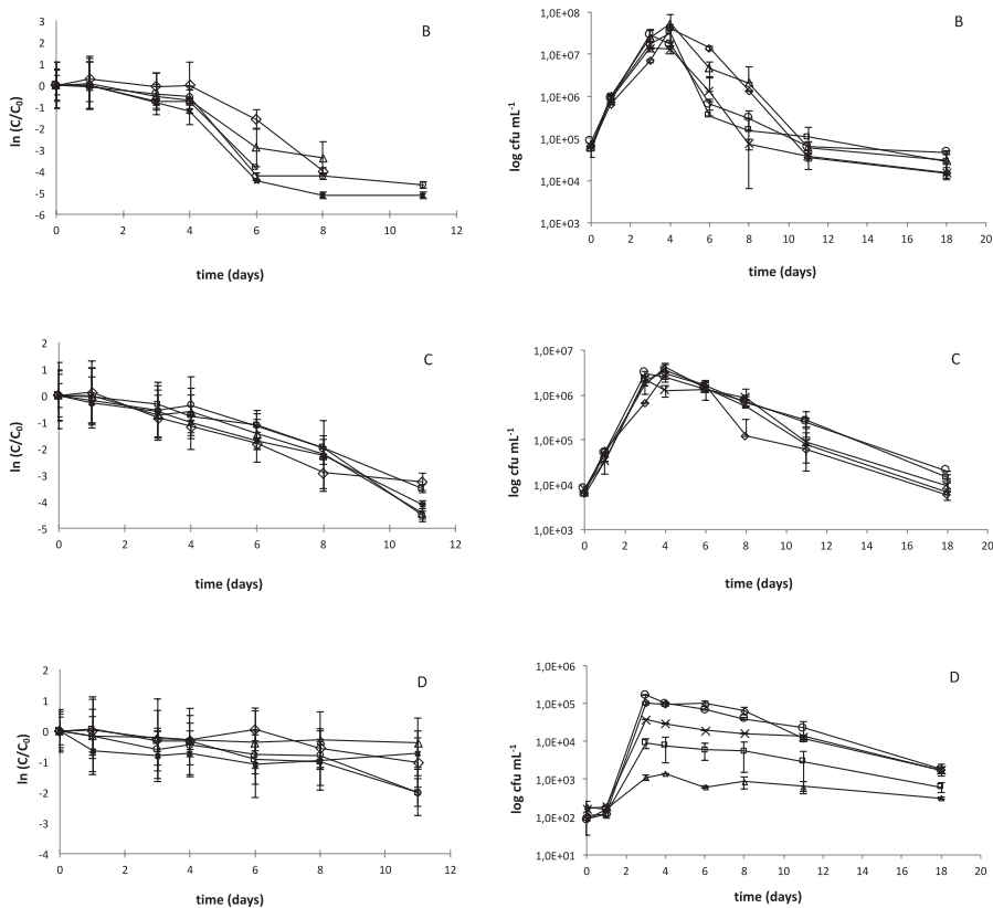
Figure 4.3. Left: Decay of Enterococcus species under conditions of competition with indigenous microbial population monitored using SBA medium: E. moraviensis ( \diamond ), E. casseliflavus ( \square ), E. hirae ( \triangle ), E. faecalis ( \circ ) and E. faecium ( \times ). Right: Total numbers of bacteria monitored using PCA medium. Signs in the right column indicate the suspension containing particular Enterococcus species. Letters refer to the plant extract concentration of 50 g L -1 (A), to 5 g L -1 (B), 0.5 g L -1 (C) and to the control measurement (D). Bars indicate standard deviations of duplicate measurements.
