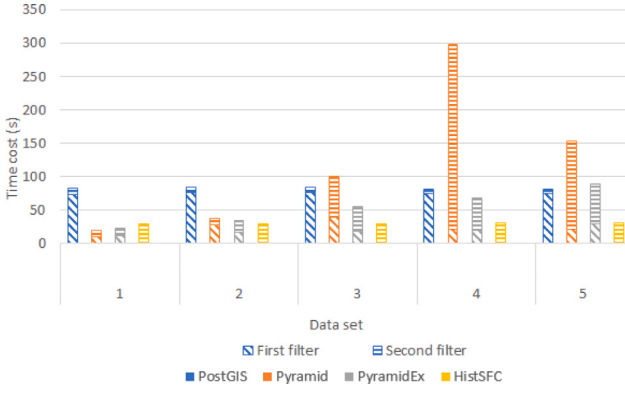
Fig. 20. Time cost of Large query using state-of-the-art solutions.
