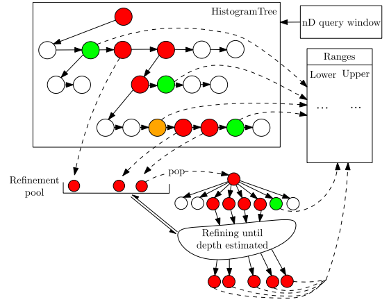
Fig. 6. Range computation using HistogramTree: with respect to the query window, green nodes are inside; red nodes are on the boundary; orange nodes are on the boundary but with few points; white nodes are outside. (For interpretation of the references to color in this figure legend, the reader is referred to the web version of this article.)
