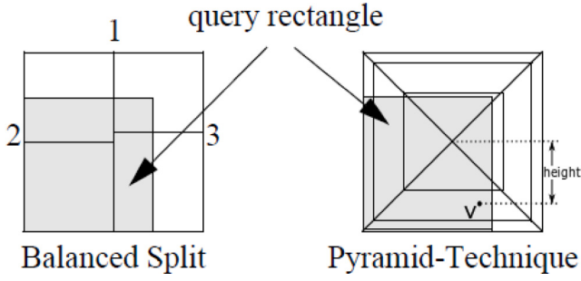
Fig. 2. Pyramid data partitioning, adapted from Berchtold et al. (1998).
