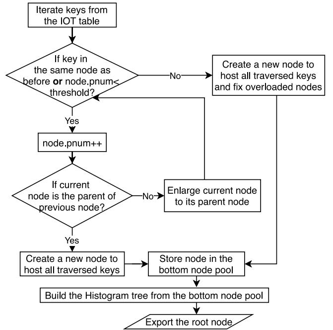
Fig. 22. HistSTREAM.
