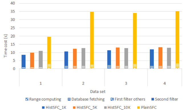
Fig. 15. Time cost of ARRIVAL24h using different HistogramTrees.
