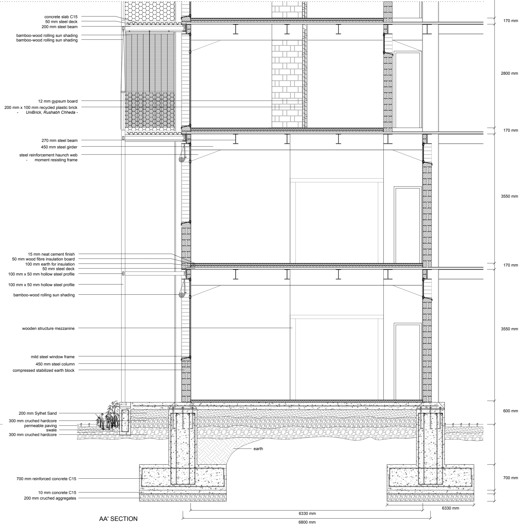
AA' SECTION
