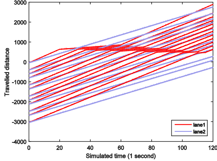
FIGURE 3. Simulated trajectories without lane change
