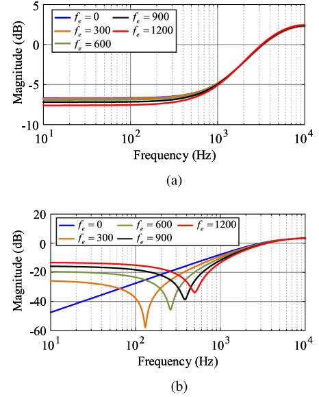
Fig. 8. Bode diagram of G_a(z) and G_b(z) when \gamma_2 is selected as (41). \delta = 0.6 and \gamma_1 = 1 . \bar{f}_{res} = 5500 Hz. f_{res} = 3875 Hz. (a) Bode diagram of G_a(z) . (b) Bode diagram of G_b(z) .
