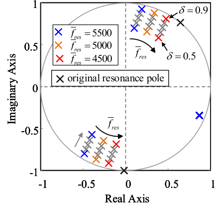
Fig. 6. Pole map of the damped model. f_e=1200 Hz. \gamma_1=1 and \gamma_2=-0.3 . f_{\text{res}}=3875 Hz.
