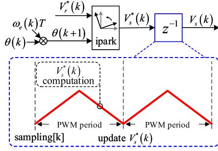
Fig. 2. Diagram of voltage reference calculation and PWM update.
