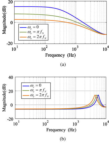
Fig. 10. Bode diagram of G_{ph}^e and G_{pl}^e when \omega_e is selected as 0, \pi f_N , and 2\pi f_N . f_N = 1200 Hz. \bar{f}_{res} = 5500 Hz. \delta = 0.8 . (a) Bode diagram of G_{ph}^e . (b) Bode diagram of G_{pl}^e .
