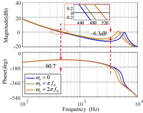
Fig. 12. Bode diagram of the open-loop transfer function with the proposed controller and the simplified coefficient selection method in (52).
