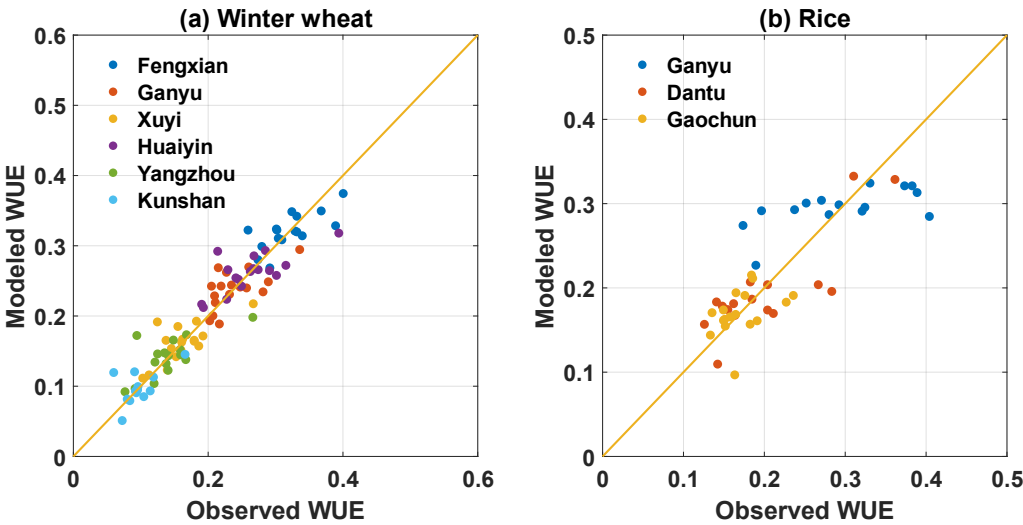
Fig. 4a, b Modeled and observed crop water use efficiency (WUE) across the stations.
