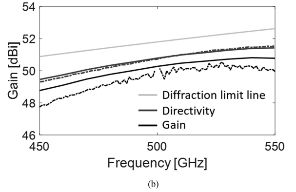
Fig. 19. Lens antenna parameters postprocessed from the coupling measurements. (a) Lens aperture efficiency and (b) gain curve. The solid curves are simulated, whereas the dash-dotted curves are postprocessed from the measurements.
