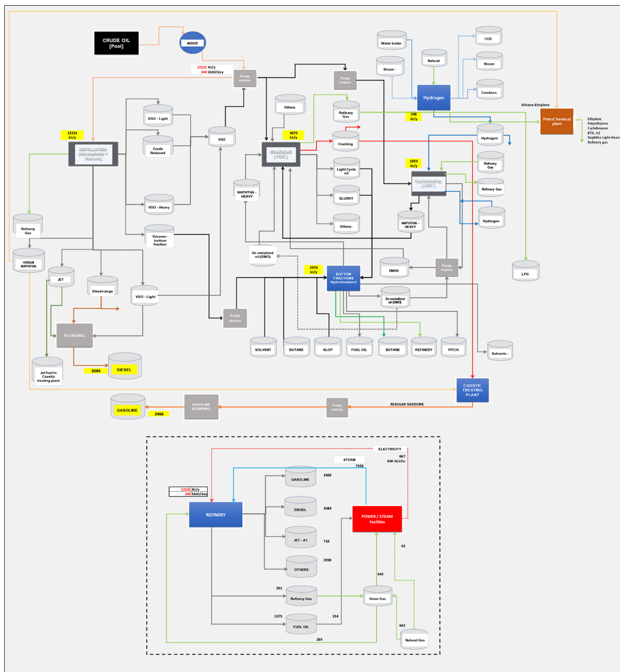
Figure 2. Schematic diagram of the refinery case study (Adapted from internal report by Ecopetro). 41
