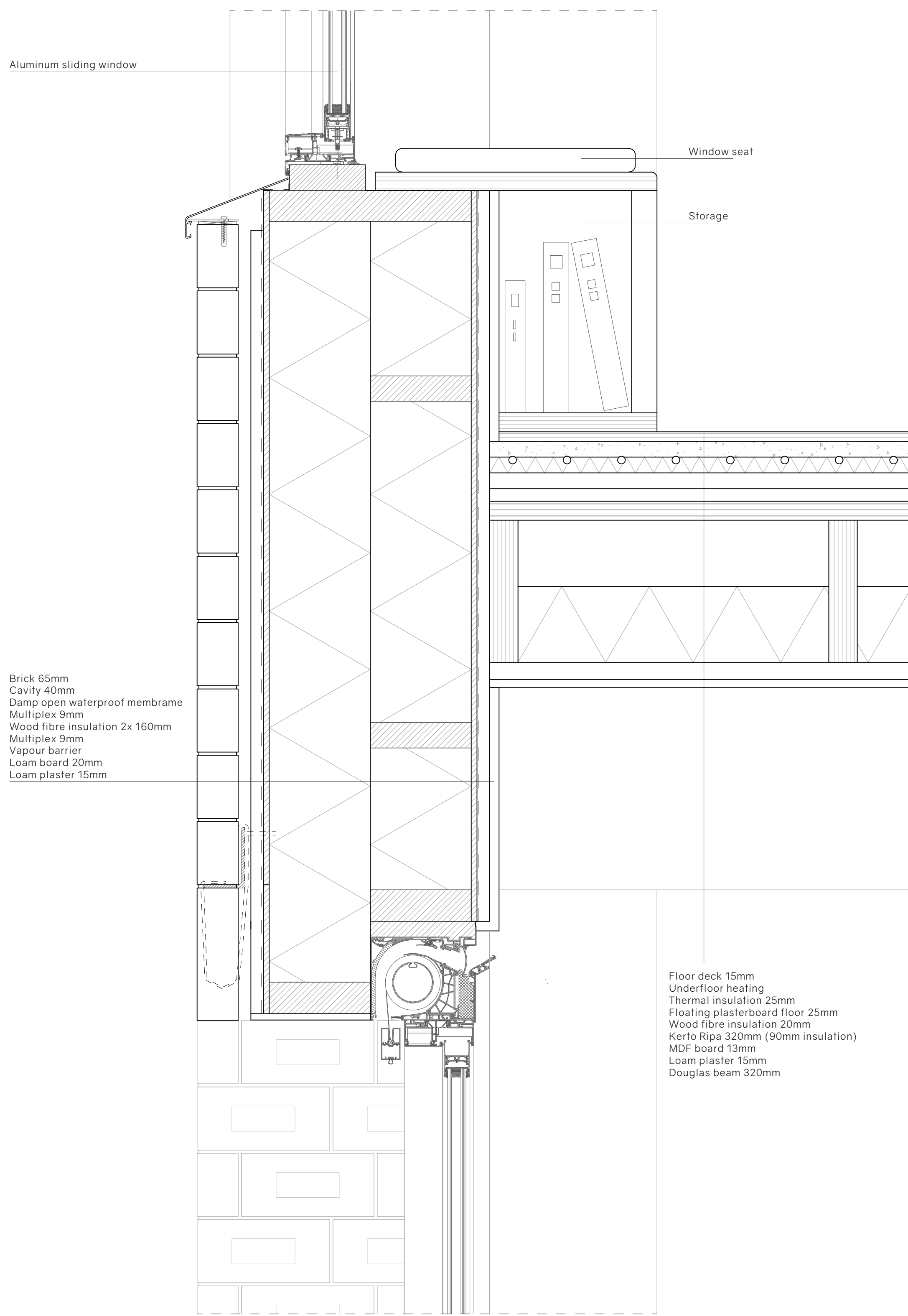
VERTICAL WINDOW DETAIL 1:5
