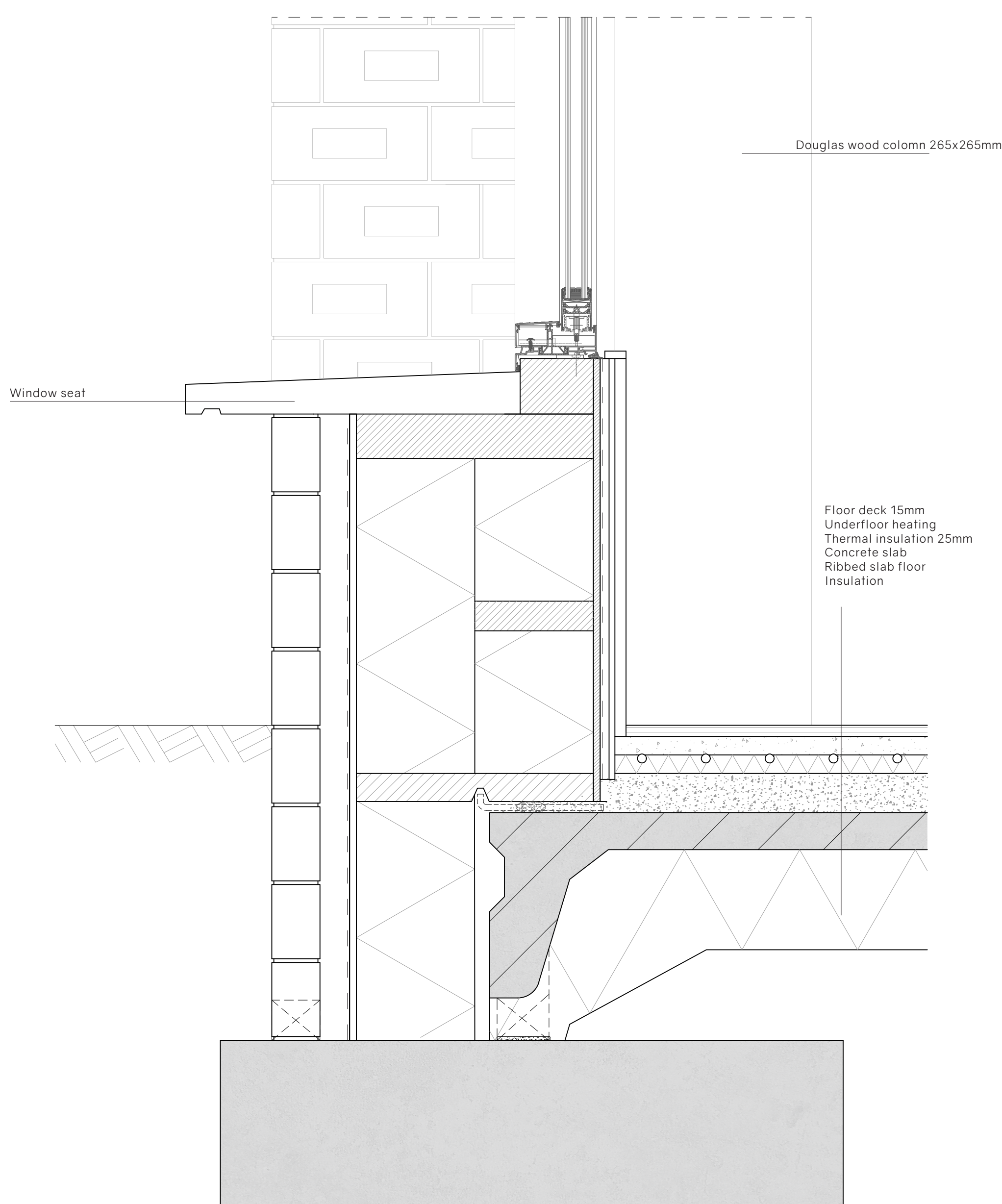
FOUNDATION DETAIL 1:5
