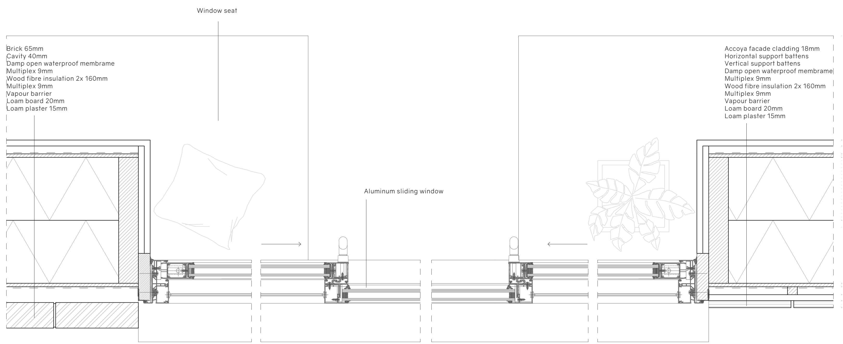
HORIZONTAL WINDOW DETAIL 1:5
