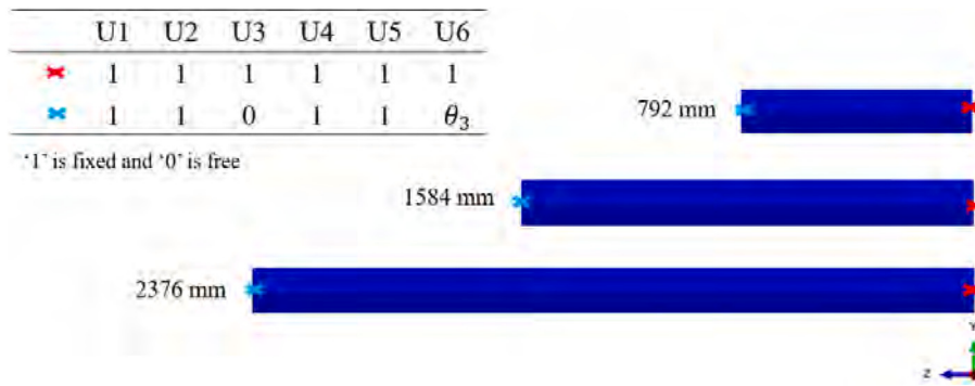
Fig. 12. Full-scale models under torsion.
