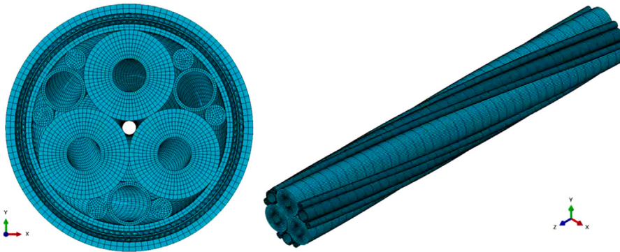
Fig. 5. The mesh results of the SPC sample.
