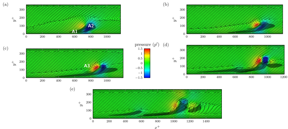
FIG. 9. Auto-generation mechanism : Vector plots of velocity ( u'^+, v'^+ ) along with fluctuation pressure ( p' ) contours in the symmetry plane which is between the two legs of an eddy. All vector are scaled by unit length, hence only indicate the flow direction. The iso-surfaces in the figures correspond the 10% of the initial maximum swirling strength. This is for two eddy case (76,51) at strength \alpha = (1, 1) with \Delta x^+ = 59 . (a)–(e) represent the evolution of two eddies and vector plots in time ( t^+ ) 28.8, 57.6, 86.4, 158.4, and 244.8, respectively.
