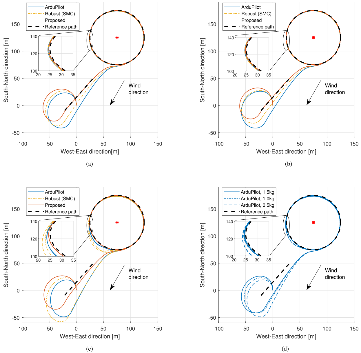
Fig. 2. Paths on the ( x - y ) plane for different masses, with original PID ArduPilot and with proposed augmentation. Note that the UAV is less affected by wind when mass=1.5 kg and more affected when mass=0.5 kg. (a) Path for mass=1kg. (b) Path for mass=1.5kg. (c) Path for mass=0.5kg. (d) Comparison of ArduPilot paths.
