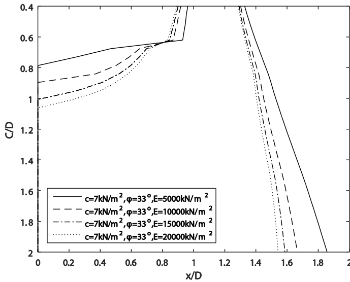
Figure 7. Effect of modulus of elasticity E on relative influence distance x/D in the case of tunnelling with D = 6\text{m}
