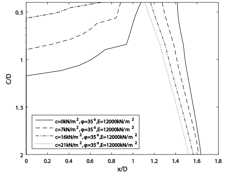
Figure 5. Effect of cohesion c on relative influence distance x/D in the case of tunnelling with D = 6\text{m}
