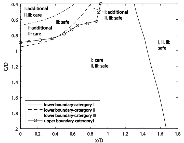
Figure 3. Relative influence distances due to tunnelling with D = 6\text{m} in clay with Risk Categories I, II, III: additional: require additional ground improvement; care: require careful control; safe: safe area with allowable settlement
