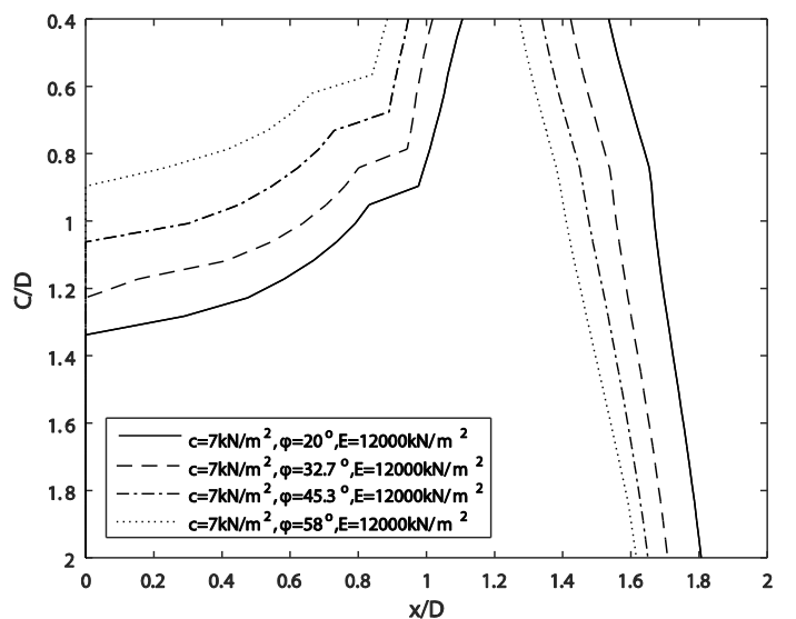
Figure 6. Effect of friction angle \phi on relative influence distance x/D in the case of tunnelling with D = 6\text{m}
