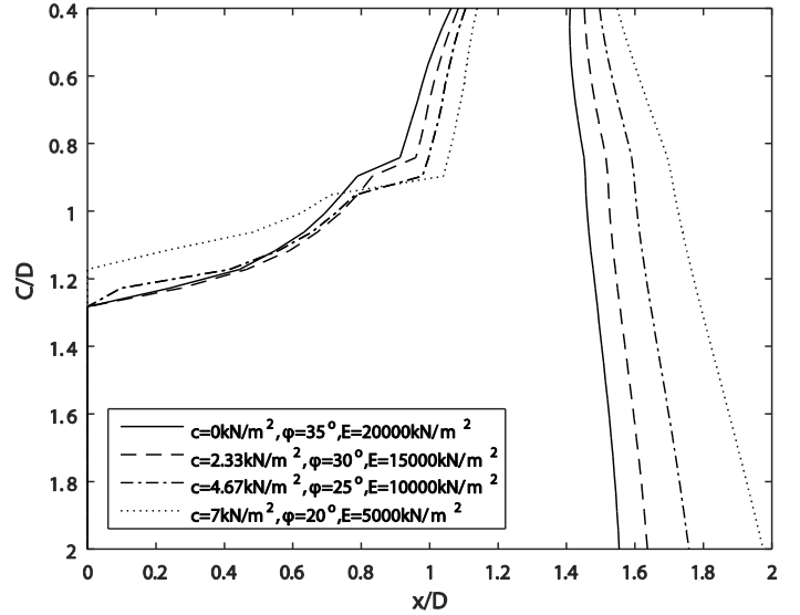
Figure 8. Combination influence of soil parameters on relative influence distance x/D in the case of tunnelling with D = 6\text{m}
