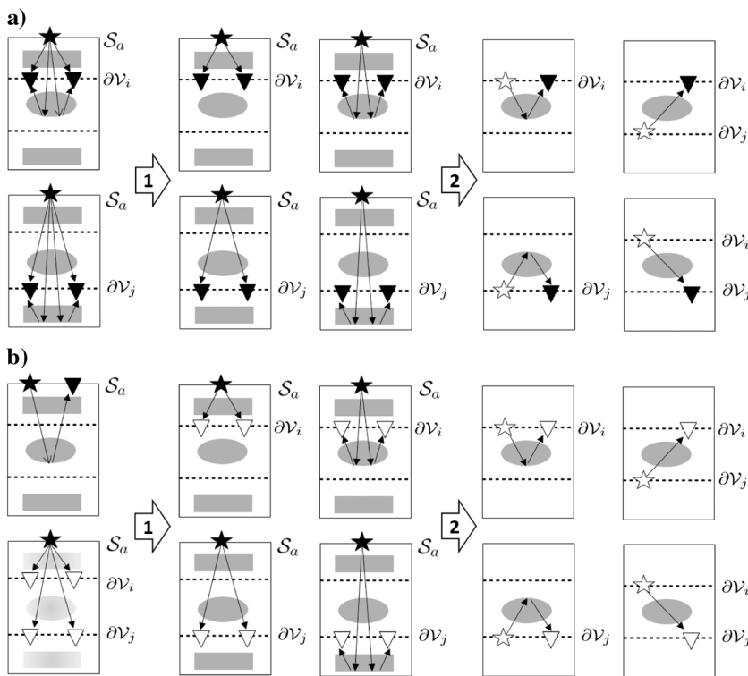
Figure 1. (a) Target-enclosed redatuming when data are physically recorded at two boundaries \partial V_i and \partial V_j . In step (1), the data are decomposed into its upgoing and downgoing constituents. In step (2), the sources are redatumed. (b) Target-enclosed redatuming when data are recorded at the acquisition boundary S_a (in the lower-left corner, we show the smooth background model). In step (1), upgoing and downgoing wavefields are retrieved, for instance, by solving the multidimensional Marchenko equation. In step (2), the sources are redatumed. Black stars and triangles represent physical sources and receivers. White stars and triangles represent virtual sources and receivers. Note that the redatumed data are defined in a reference medium, which is reflection-free above \partial V_i and below \partial V_j , but identical to the physical medium in between these boundaries.
