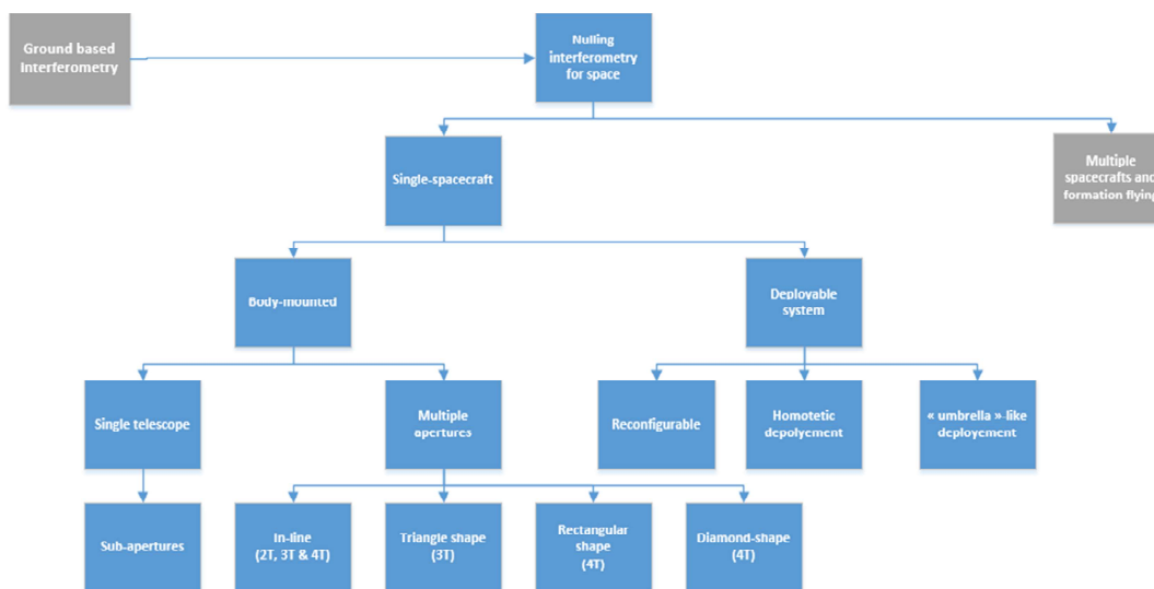
Figure 1: Summary of the nulling interferometry concepts useful for space and under study.
