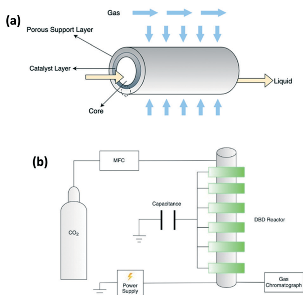
Fig. 8 Schematic representation of (a) membrane microreactor; and (b) microwave reactor set-up.
