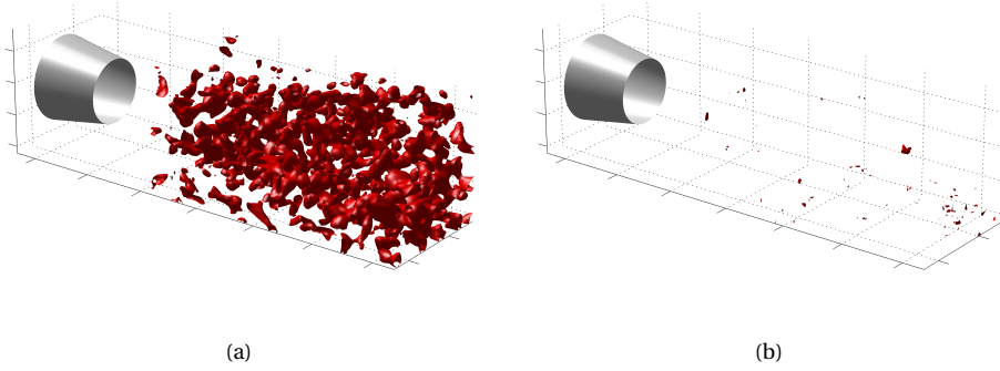
Figure 3.7: Circular jet in water: isosurfaces of velocity divergence at 15 1/s of the original data set (a) and after applying SGPR (b).
