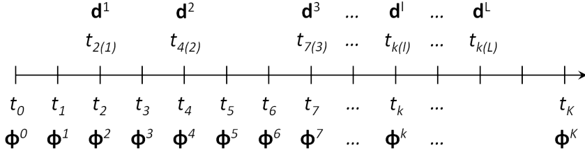
Figure 2.3: Discretization of the state \phi^k and the availability of the measurements d^l in time (adapted from Evensen (2009)).
