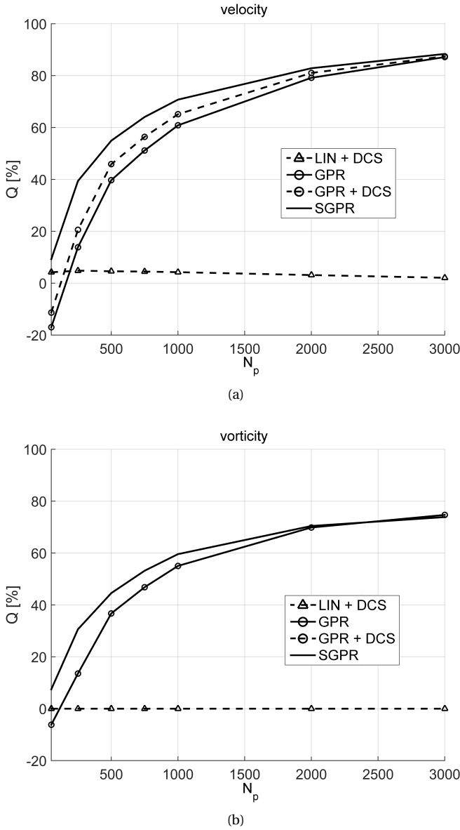
Figure 4.6: The vortex ring: improvement with respect to linear interpolation ( Q ) as a function of number of measurement points ( N_p ) for the velocity (a) and vorticity (b) fields.
