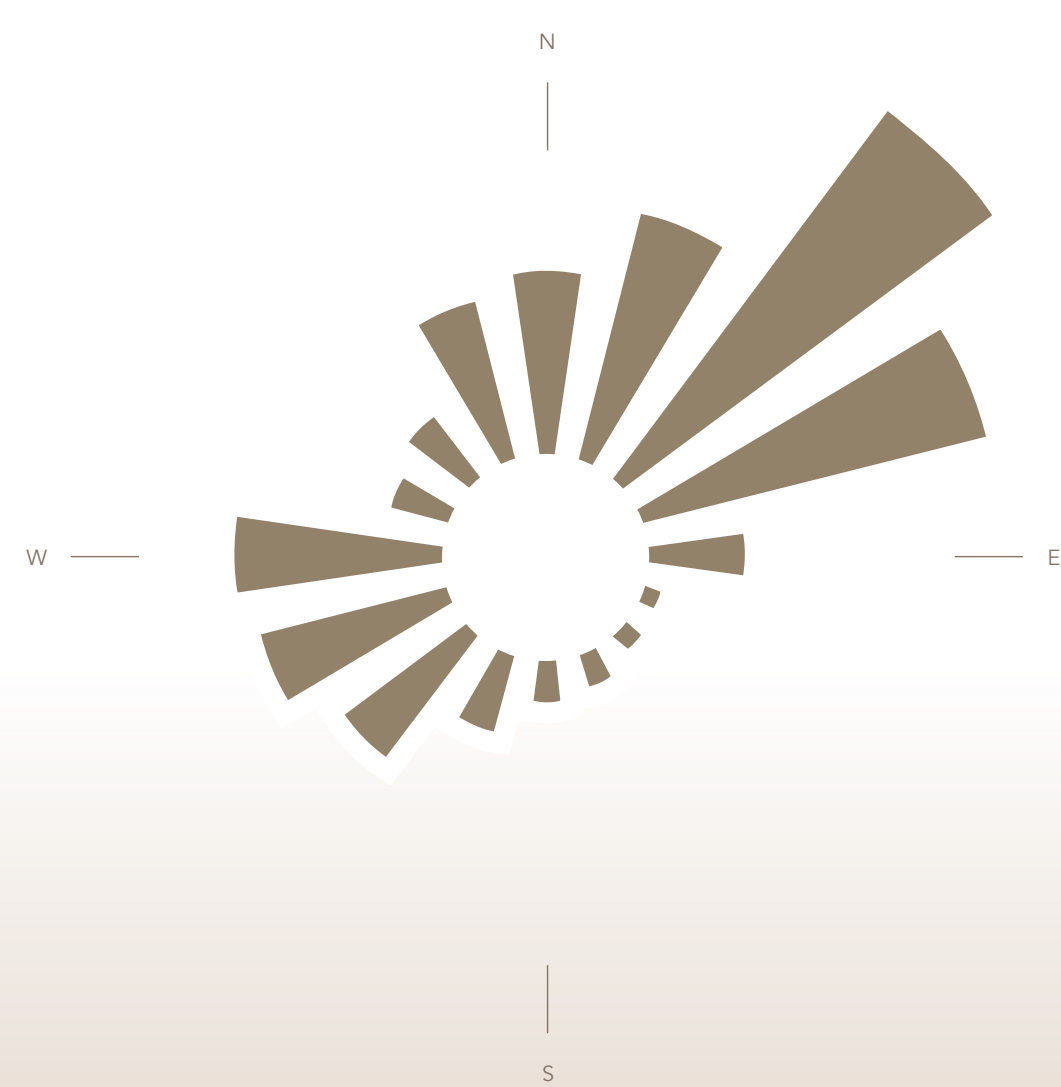
wind rose I Muscat Seeb
