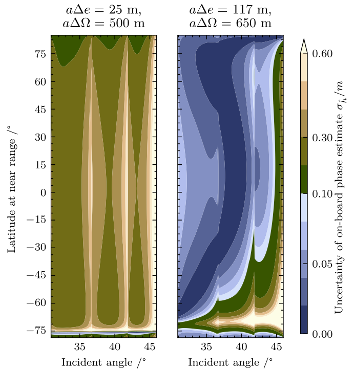
Fig. 15. Uncertainty of the phase estimate due to the along-track separation in terms of 1\sigma at a wind speed of 5 \text{ ms}^{-1} . The ATI phase estimate \phi_{\text{ATI}} is obtained using the two phase centers onboard each Harmony companion.
